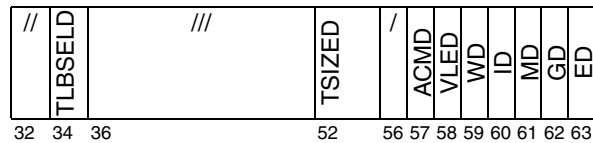
Figure 46. MAS4 register [MAV=1.0]
