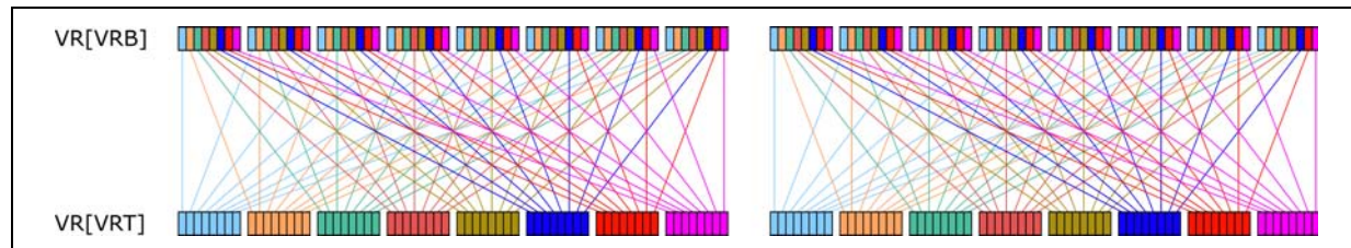
Figure 70. Vector Gather Bits by Bytes by Doubleword
