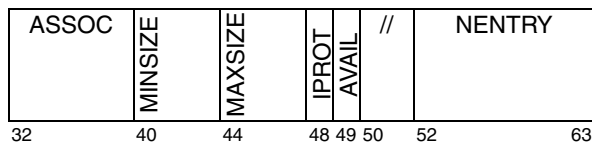
Figure 30. TLB Configuration Register [MAV=1.0]
